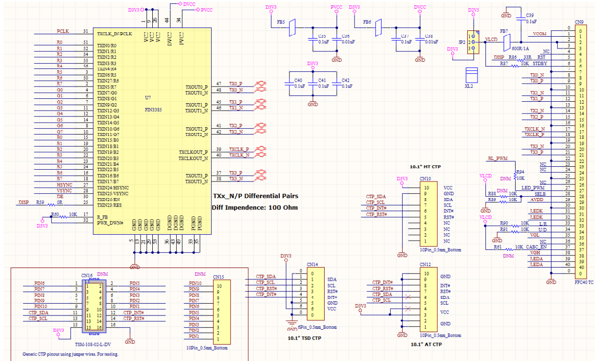
Figure 4-3 - Host Interface Connectors
